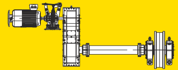
2T - Open winch and cranes
